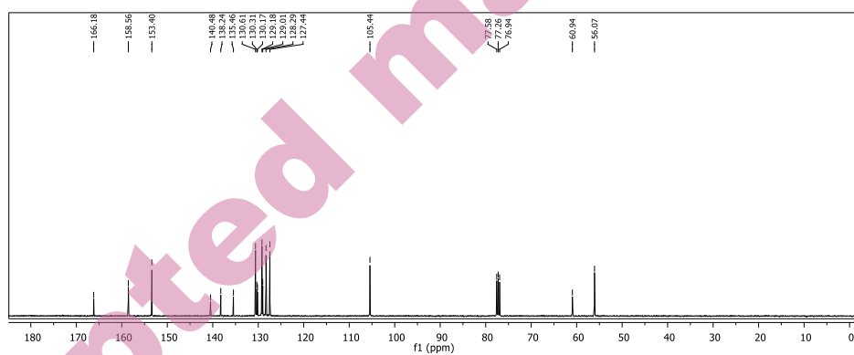
Figure S6. 13 C NMR spectrum of 1-(diphenylmethylene)-2-(2,3,4-trimethoxybenzylidene)hydrazine ( 7 ) in CDCl 3
