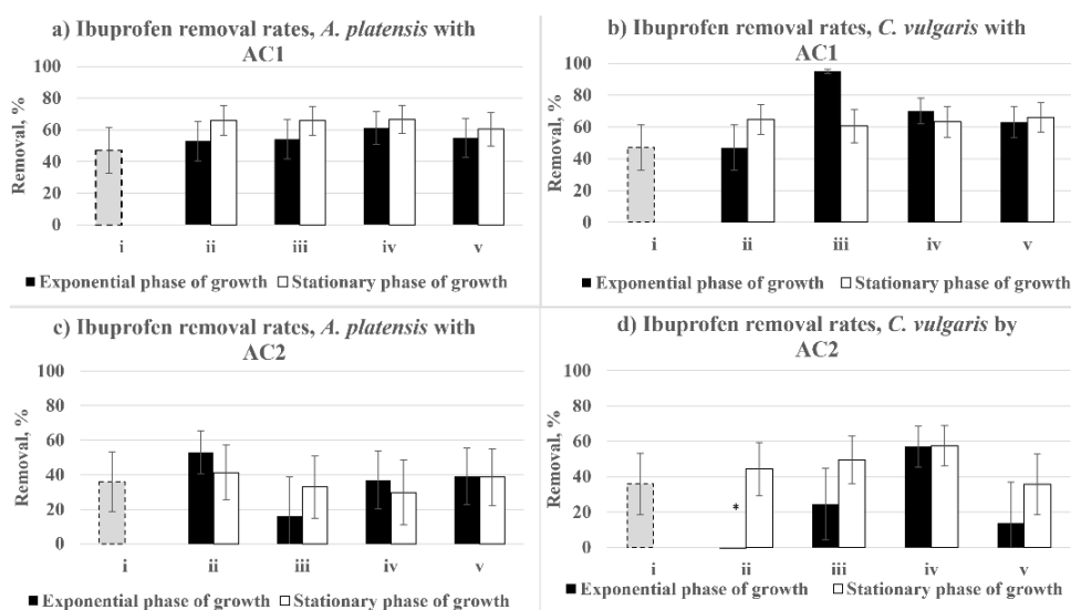
Fig. 1. Efficiency of IB removal using PACs (dose 5 mg L -1 ). i ) DCTW without microalgae addition (average value of five replicates); ii ) non-chlorinated matrix with tAOM; iii ) non-chlorinated matrix with dAOM; iv ) pre-chlorinated with tAOM; v ) pre-chlorinated with dAOM. * – No removal efficiency; Letters a–d indicate ibuprofen removal rates for A. platensis with AC1 (a), C. vulgaris with AC1 (b), A. platensis with AC2 (c) and C. vulgaris with AC2 (d). Error bars show the error of the relative removal. The number of cells in matrices containing A. platensis in exponential and stationary phase of growth were 8 \times 10^8 and 4 \times 10^8 cells L -1 , respectively. For C. vulgaris these numbers in exponential and stationary phase of growth were 2 \times 10^8 and 5 \times 10^8 cells L -1 , respectively.
