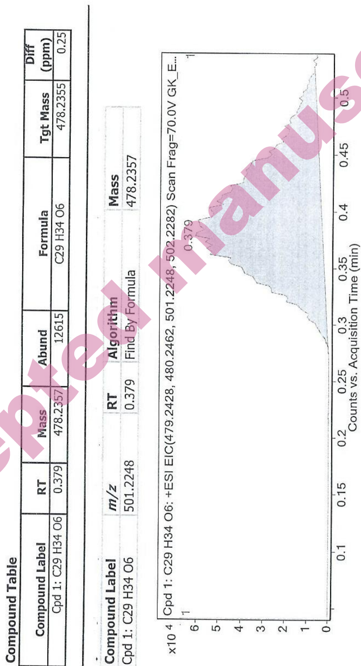
Figure S7: HRMS data of compound 1
