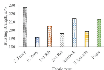
Fig. 3. Impact of internal notation on bursting strength.
