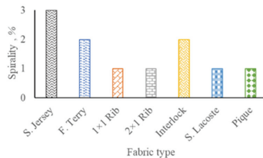
Fig. 5. Impact of internal notation on spirality.
