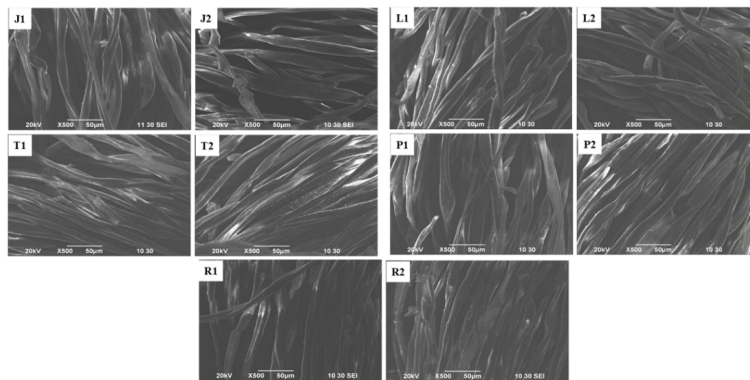
Fig. 2. SEM photographs of S. Jersey fabric: before (J1) and after c(J2) oloration; Frence Terry fabric: before (T1) and after (T2) coloration; 1×1 Rib fabric: before(R1) and after (R2) coloration; Lacoste fabric: before(L1) and after (L2) coloration; Pique fabric: before (P1) and after (P2) coloration.
