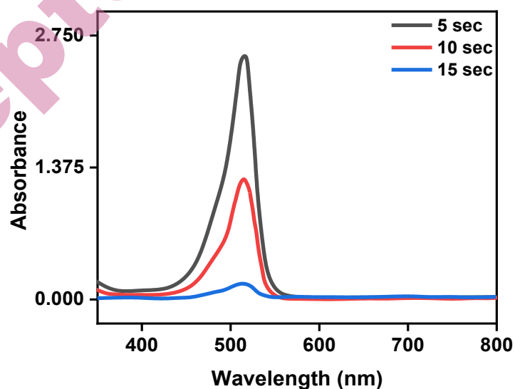
Fig. 5. UV-Vis spectra of dye degradation
