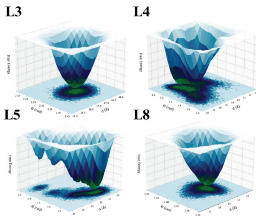
339 Fig. 4. Free-energy landscapes for best binding ligands (L3, L4, L5, L8). 340
