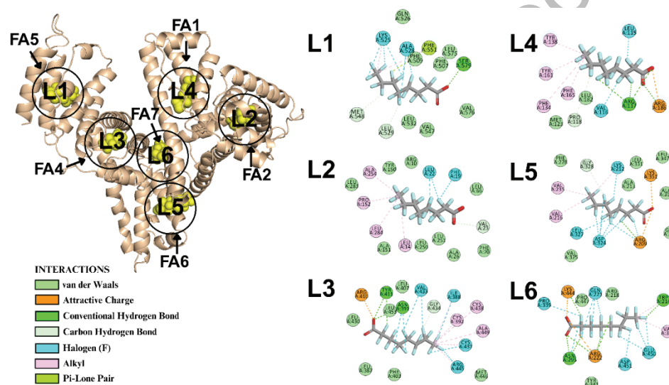
196 Fig. 1. Left: 3D structure of HSA with PFOA bound at the six top-scoring docking positions. 197 Right: 2D interaction diagrams between HSA residues and PFOA for these positions. 198
