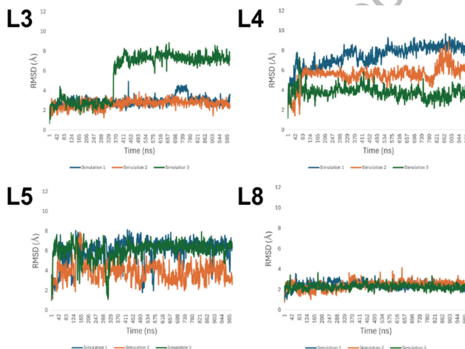
323 Fig. 3. RMSD plots for the four ligands of interest (L3, L4, L5 and L8) during 1,000-ns 324 MD simulations. 325
