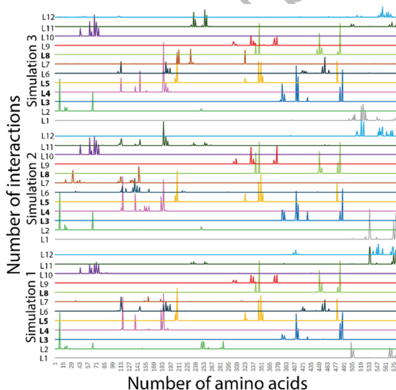
266 Fig. 2. Ligand–residue interaction maps (LRIMs) for ligands L1–L12 from three MD simul- 267 ations. The x-axis shows amino acid positions, the y-axis the number of frames with contacts. 268 Different colors mark individual ligands; peaks indicate residues frequently involved in 269 binding. 270
