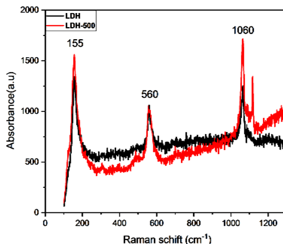
Fig. 3. Raman spectra of LDH and LDH-500 samples.
