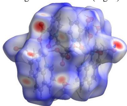
Fig. 4. Three-dimensional Hirshfeld surface of 1 mapped with dnorm.
