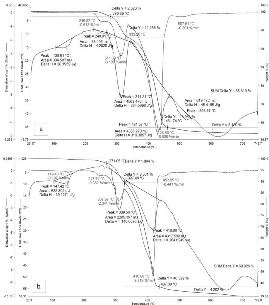
Fig. 5. Thermal analysis results for AH 45 Bt 5 (a) and AH 25 Bt 25 (b) polymer composites.
