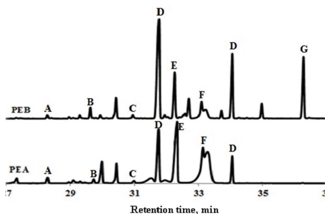
Fig. 2. Monosaccharide chromatogram of polysaccharidic extracts of Isochrysis galbana (PEA) and Nannochloropsis oculata (PEB) determined by trimethylsilylation method. A: xylose; B: mannose; C: galactose; D: glucose; E: sorbitol; F: mannitol; G: inositol.
