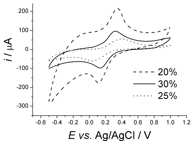
Figure S-1. Effect of TCP mass fraction in CPE/CHTCN 0.1 on cyclic voltammograms of Fe(CN) 6 3-/4- redox couple in 0.1 M K 2 SO 4 .
