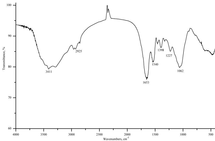
Fig. S-2. FTIR spectrum of S. fradiae biomass after MB biosorption.
