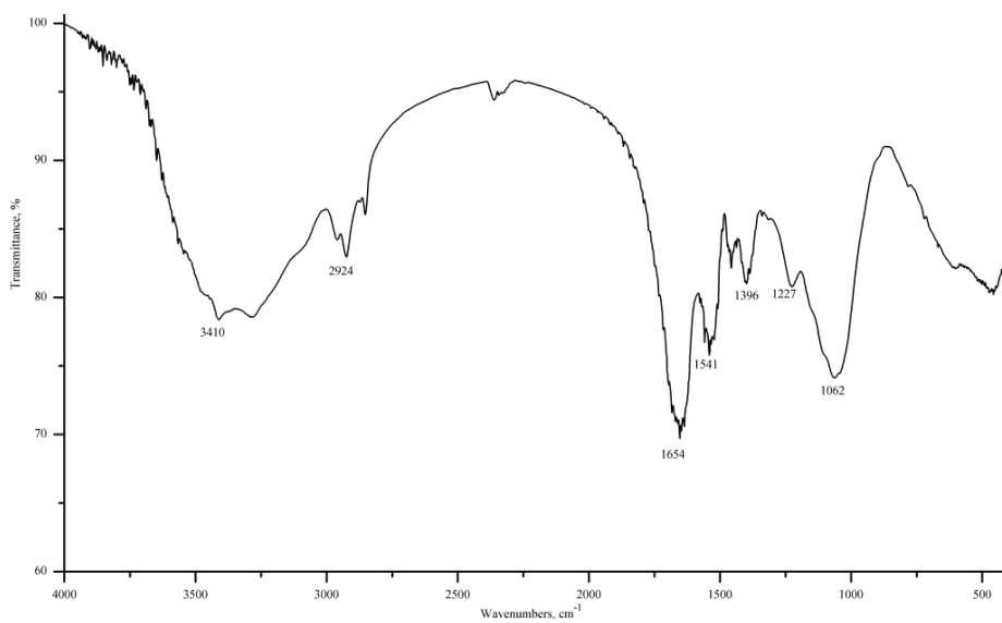
Fig. S-3. FTIR spectrum of S. fradiae biomass after CR biosorption.
