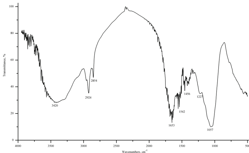
Fig. S-1. FTIR spectrum of waste pretreated Streptomyces fradiae biomass.
