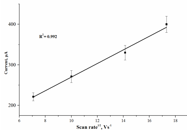
Figure S 2. Peak current vs square root of scan rate ( v^{1/2} )
