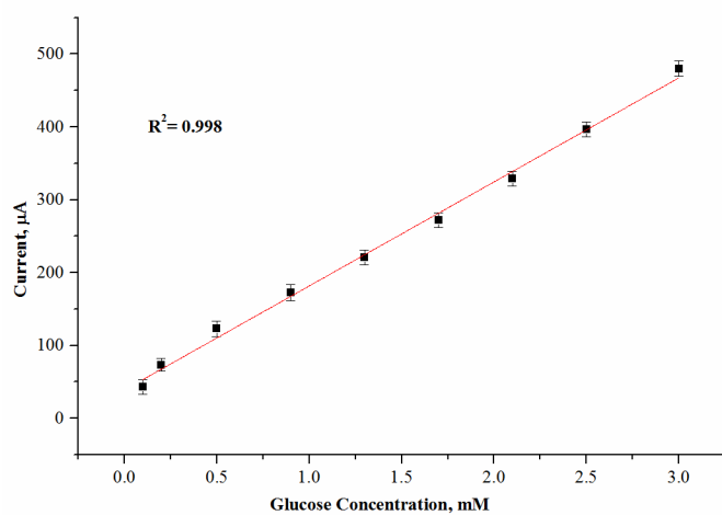
Figure S 1. Peak current ( I_p ) vs concentration
