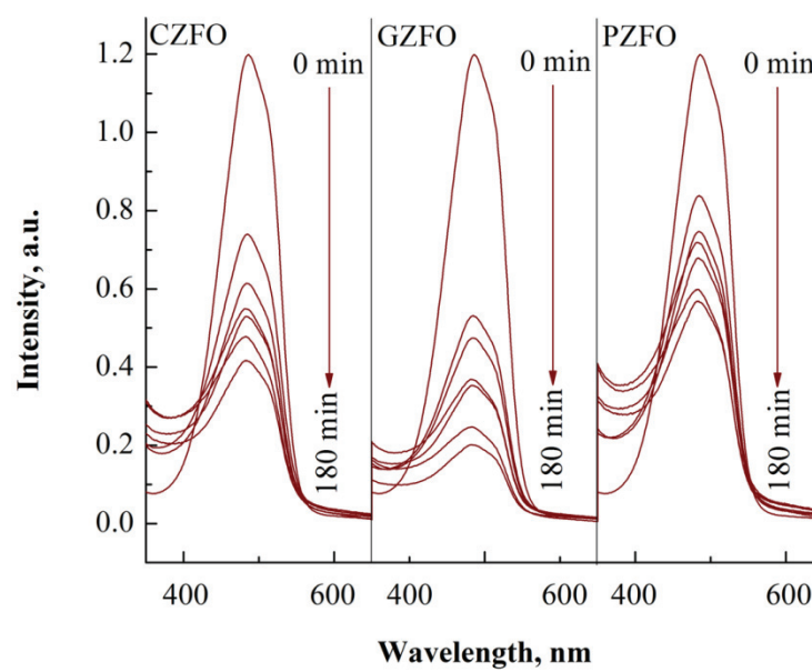
Fig. S-4. UV-Vis absorption spectra of MO solution after different reaction periods over different samples.
