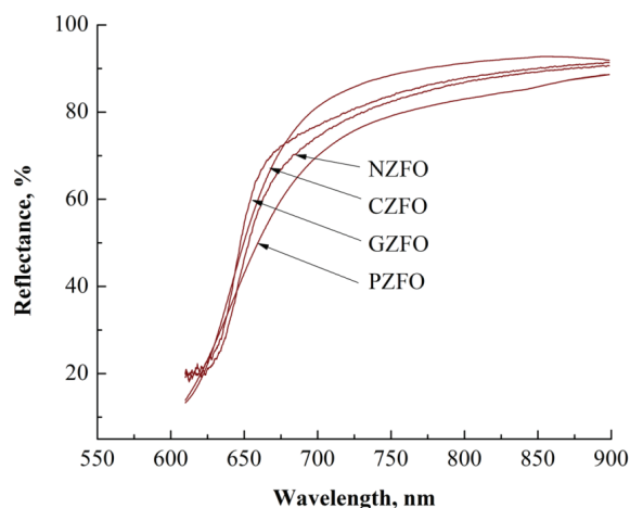
Fig. S-2. UV-Vis DRS spectra of the obtained samples.
