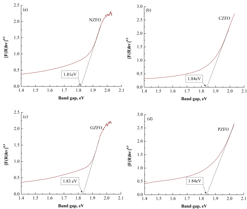
Fig. S-3. The relationships between [F(R) \cdot hv]^{0.5} and band gap of: a) NZFO, b) CZFO, c) GZFO and d) PZFO.
