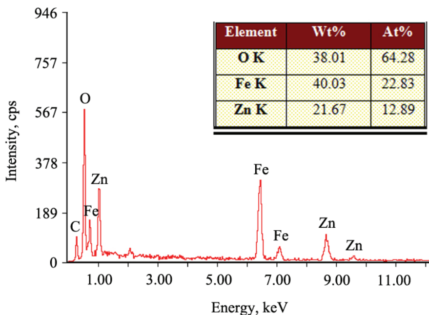
Fig. S-1. EDS pattern of NZFO sample.
