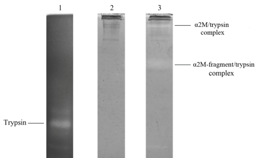
Fig. S-1. Trypsin zymography of trypsin alone (A), \alpha_2 M alone (B) and a sample of mixed \alpha_2 M and trypsin (C).
