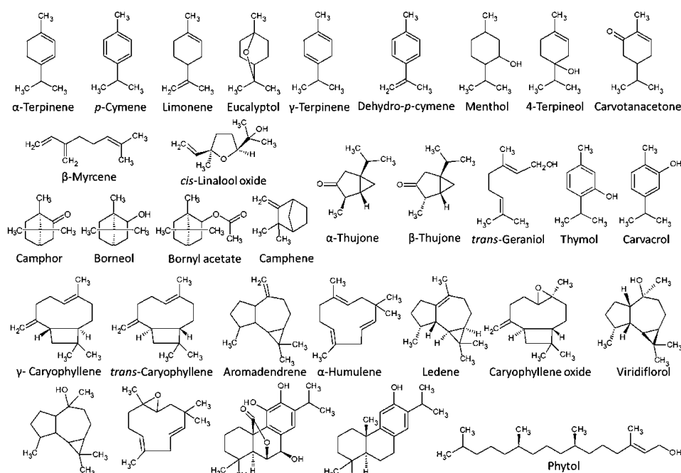
Fig. S-1. Detected terpenoids in sage essential oil obtained by supercritical fluid extraction.
