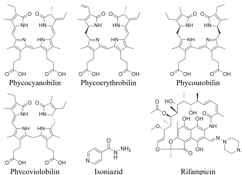
Scheme 1. Structures of phycocyanobilin, phycoerythrobilin, phycourobilin, phycoviobobilin, isoniazid and rifampicin.
